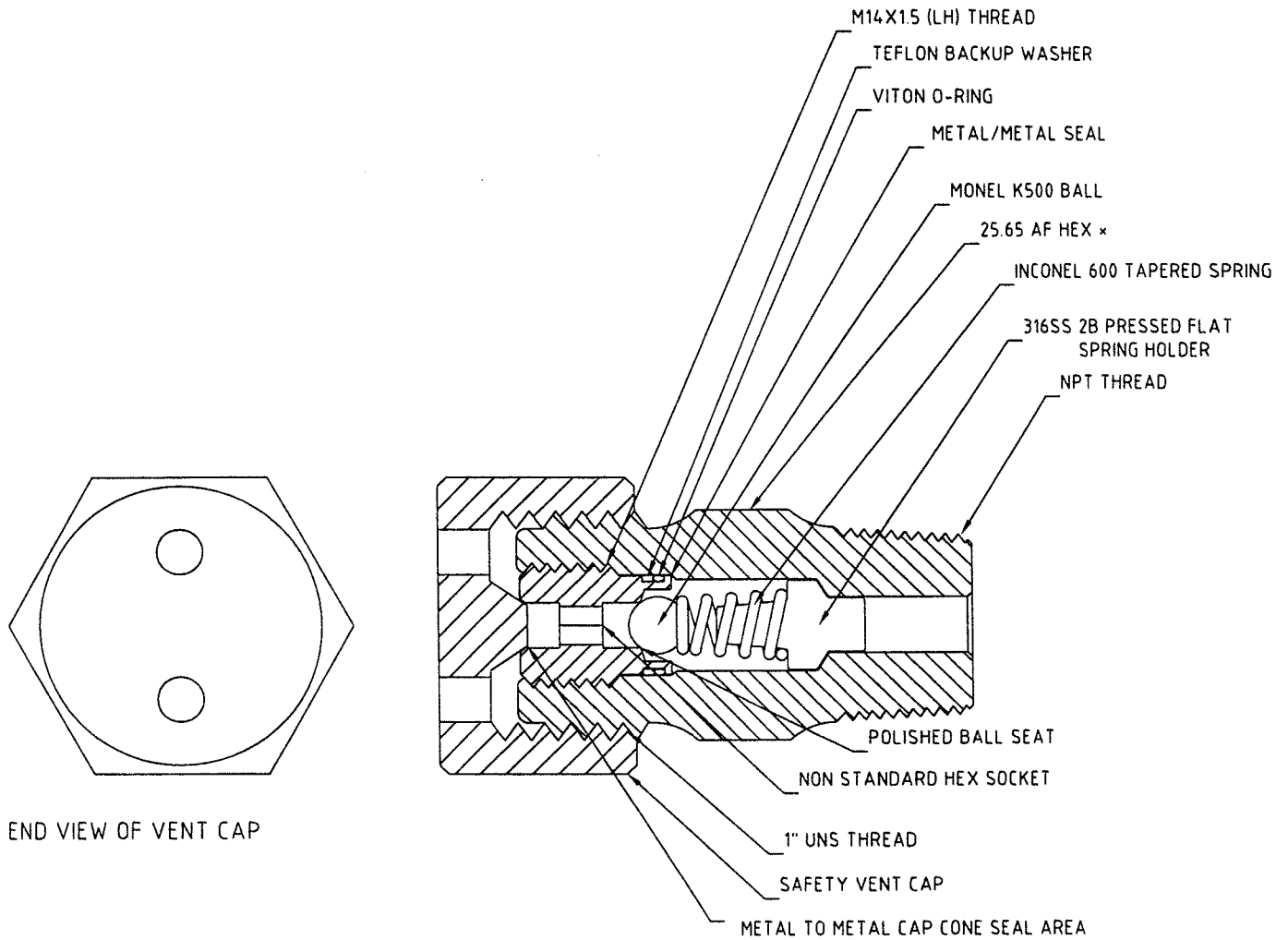
ASSEMBLY DRAWING
